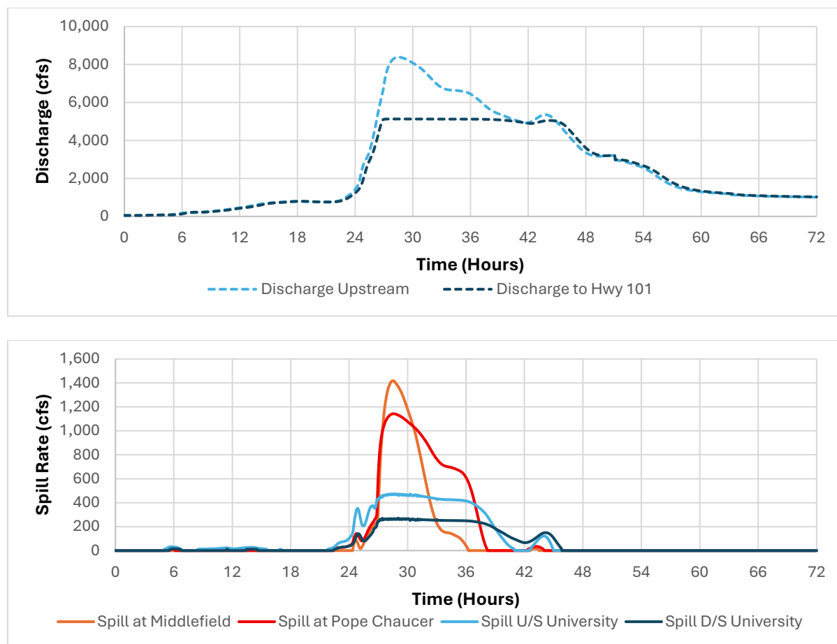
Figure 5-15: 100-Year Design Storm Hydrographs
