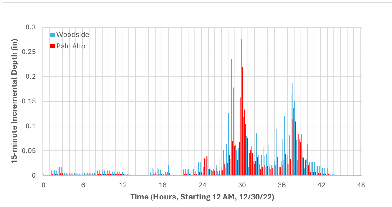
Figure 3-1: NYE22 Rainfall Timeseries Used in the ICM
