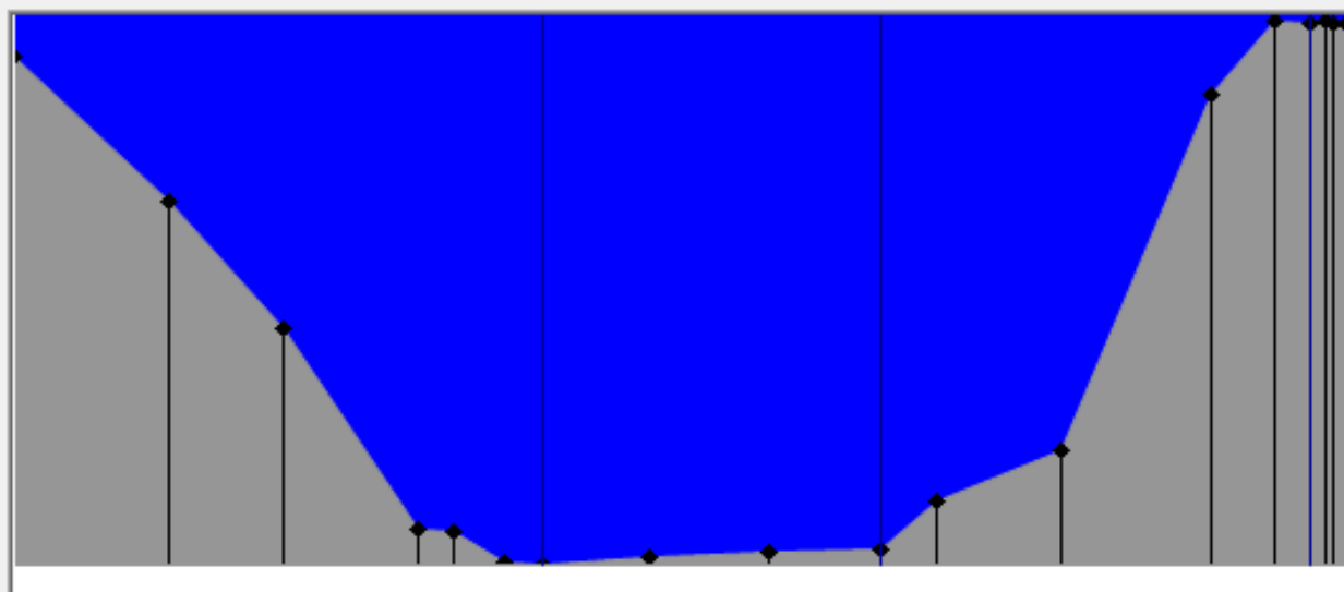
Figure 4-16: Example Cross Section from the Model Update
