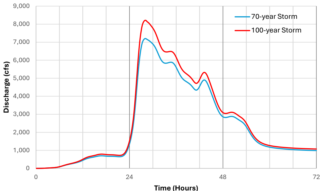
Figure 3-9: Design Storm Discharge Hydrographs at Stanford Gage
