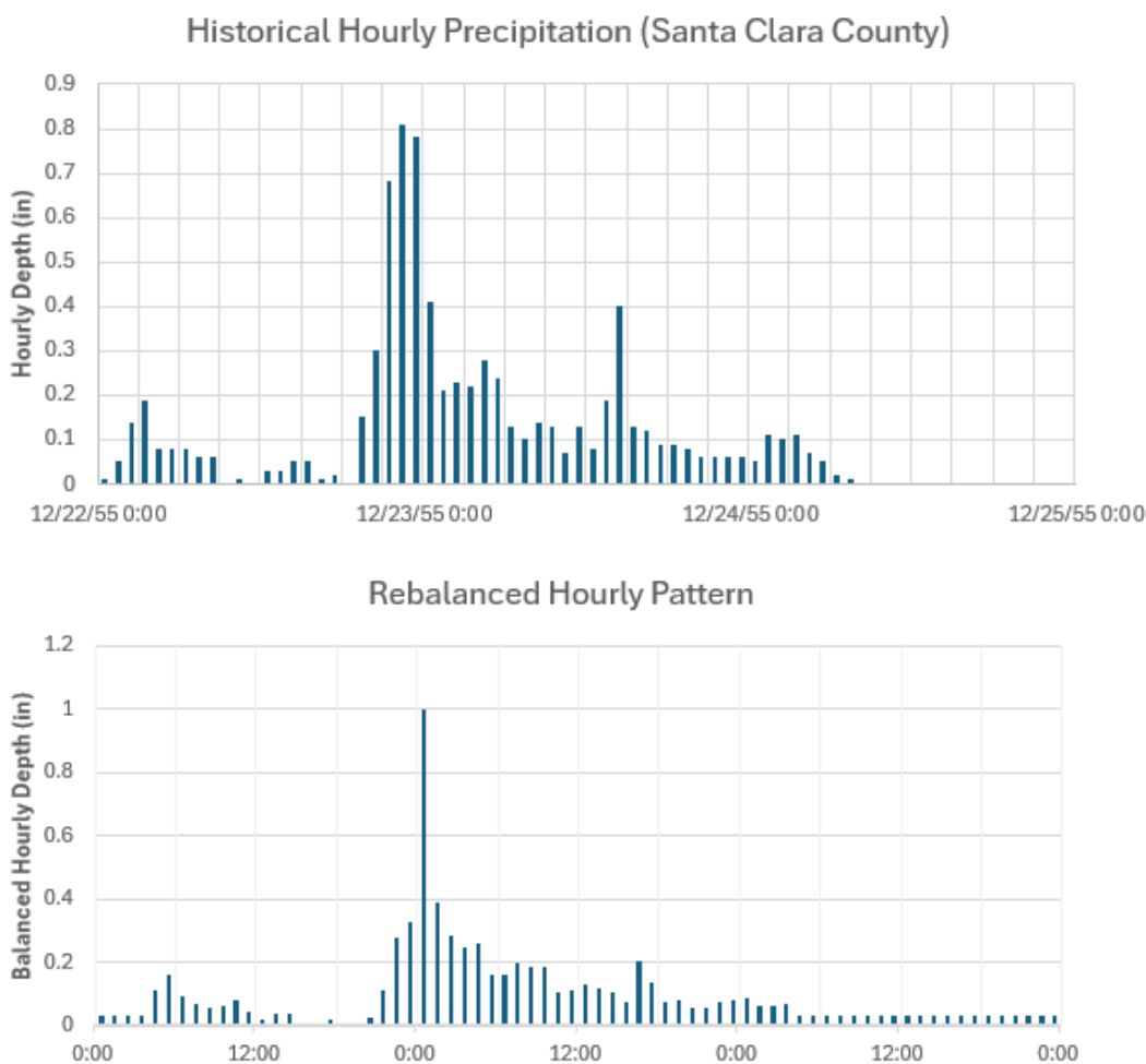
Figure 3-2: December 1955 Precipitation (Top) Rebalanced with Local Statistics (Bottom)
