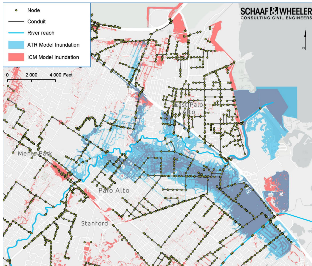
Figure 6-2: Overlay of 100-year ATR Model Inundation with ICM Inundation
