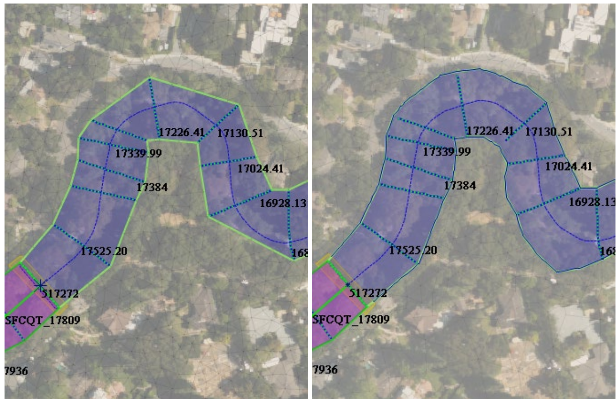
Figure 4-13: River Reach and Bankline Layout
