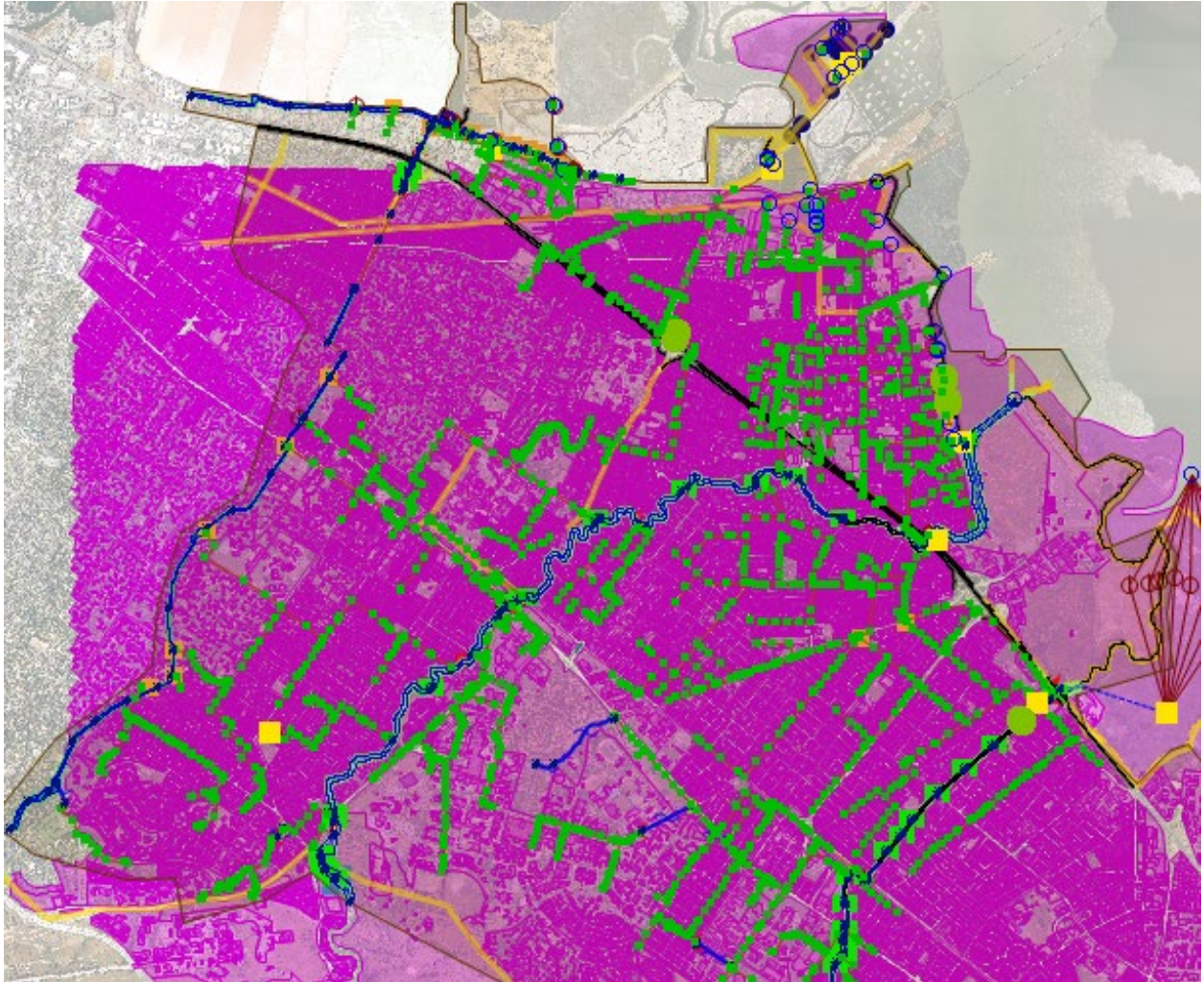
Figure 4-8: Expanded Model Mesh Area with Enlarged Roughness Zone Layer
