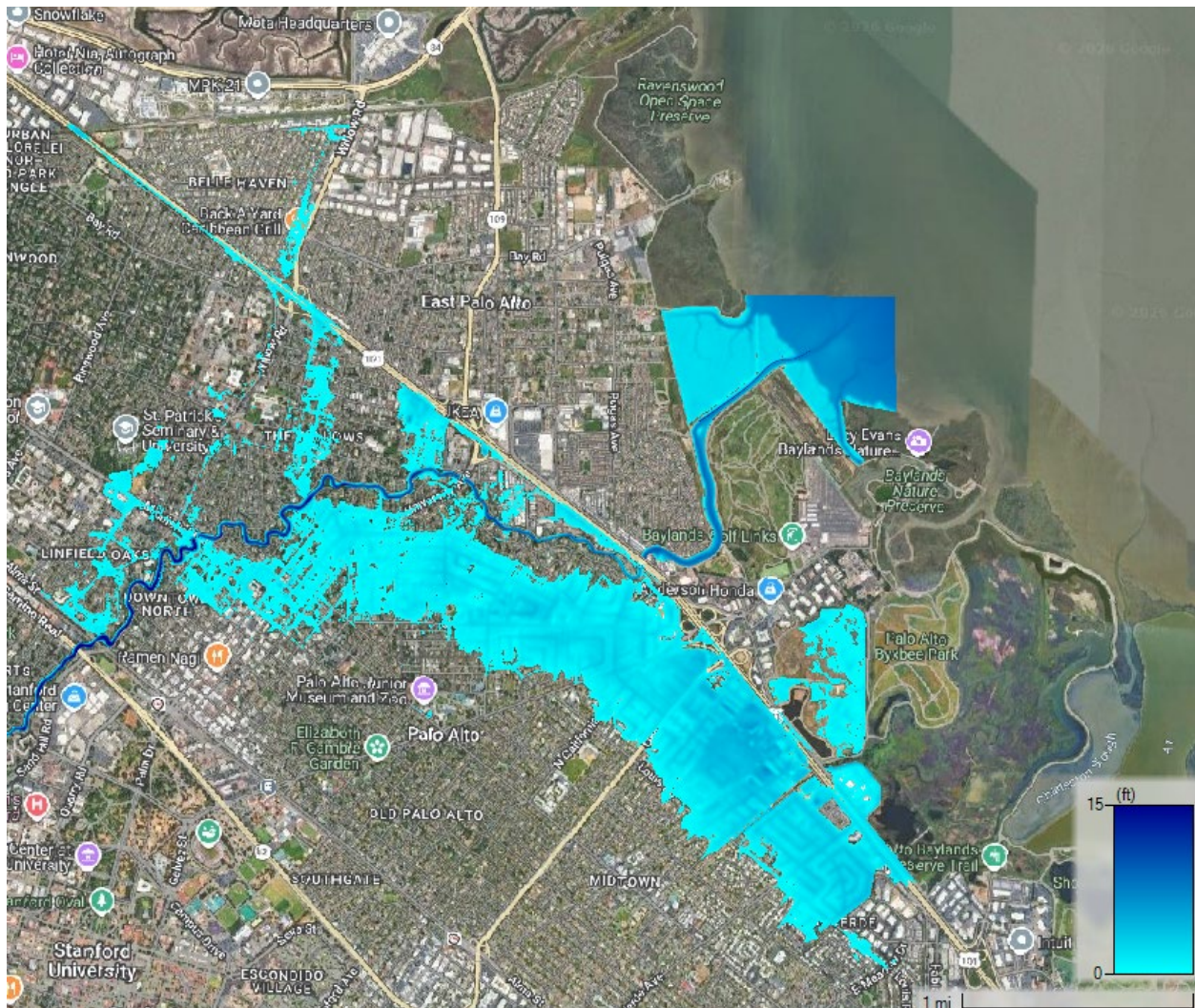
Figure 6-1: 100-year Updated HEC-RAS Model Result (Maximum Depth)
