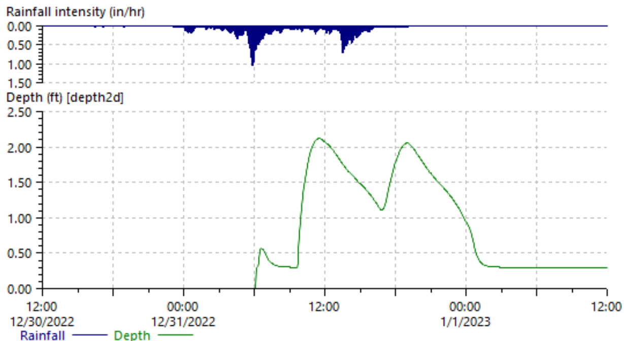
Figure 5-10: Modeled Rainfall and Flood Depth at West Bayshore Road
