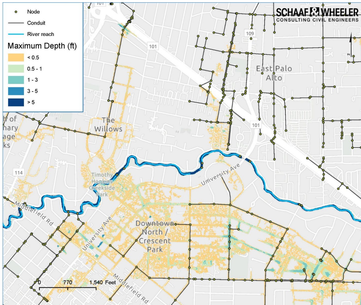
Figure 5-4: NYE22 Modeled Inundation Comparison
