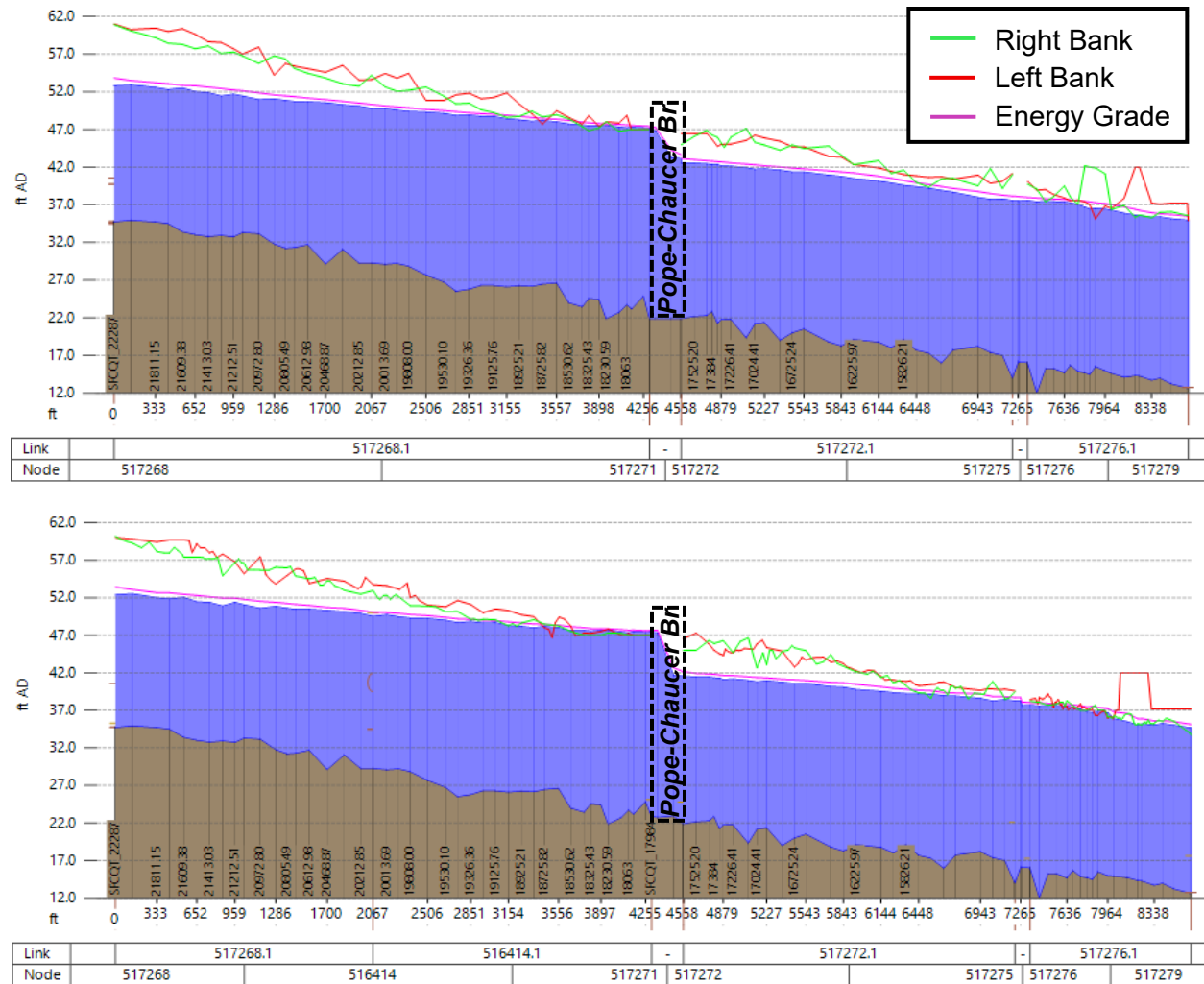
Figure 5-1: Comparison of NYE22 Profiles Between ICM Versions
