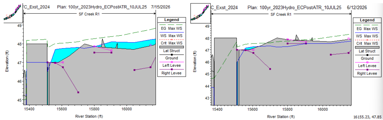
Figure 6-3: Results at Pope-Chaucer for the ATR Run (Left) and with Corrected HTab Inputs (Right)
