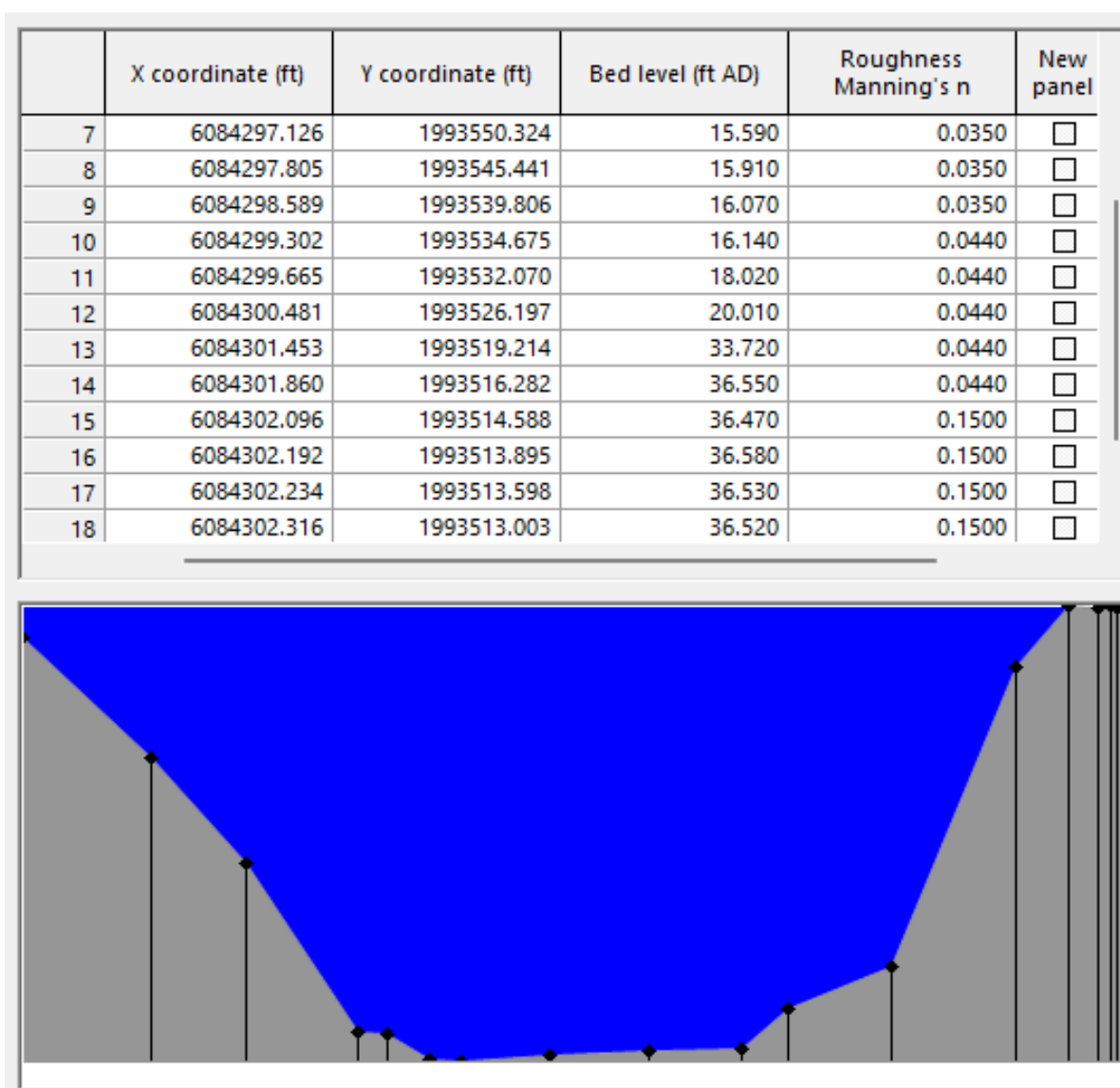
Figure 4-15: Example Cross Section Imported to 2023 ICM from the Calibrated HEC-RAS Model
