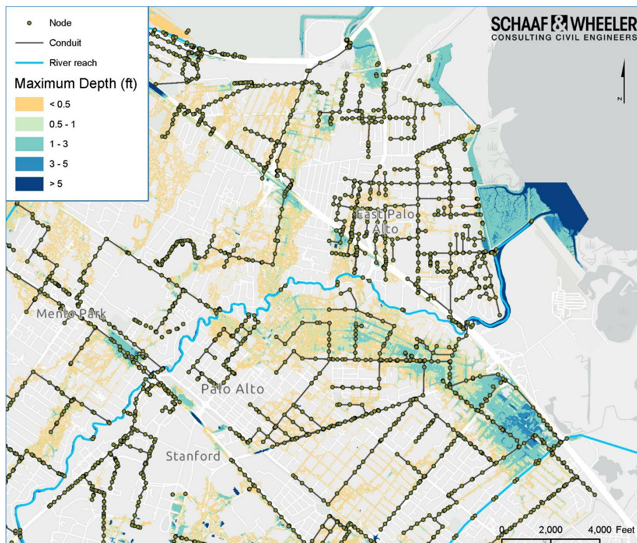
Figure 5-12: 70-year (7,200 cfs) Design Flood Depths
