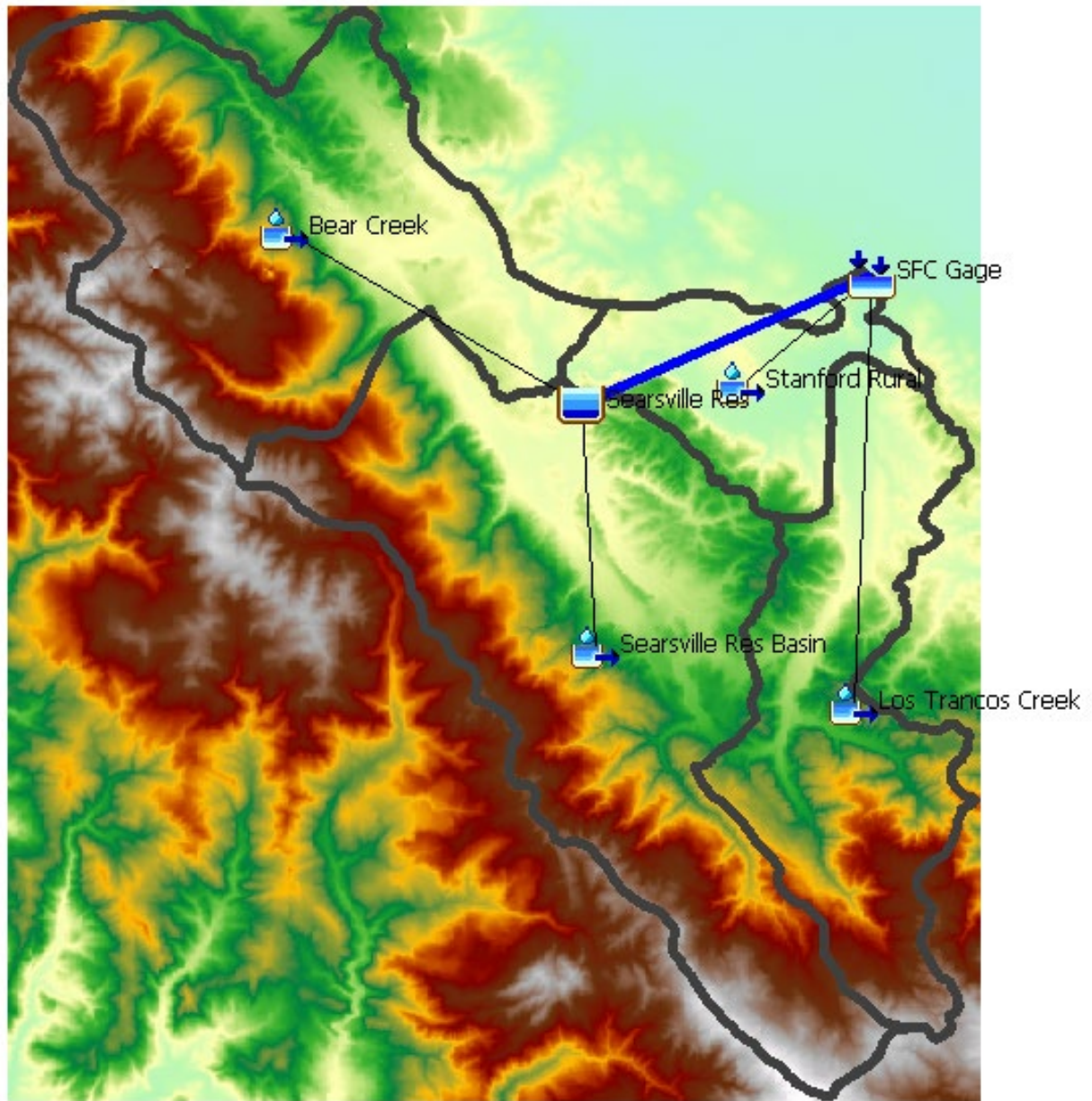
Figure 3-6: HEC-HMS Calibration at Stanford Gauge Location
