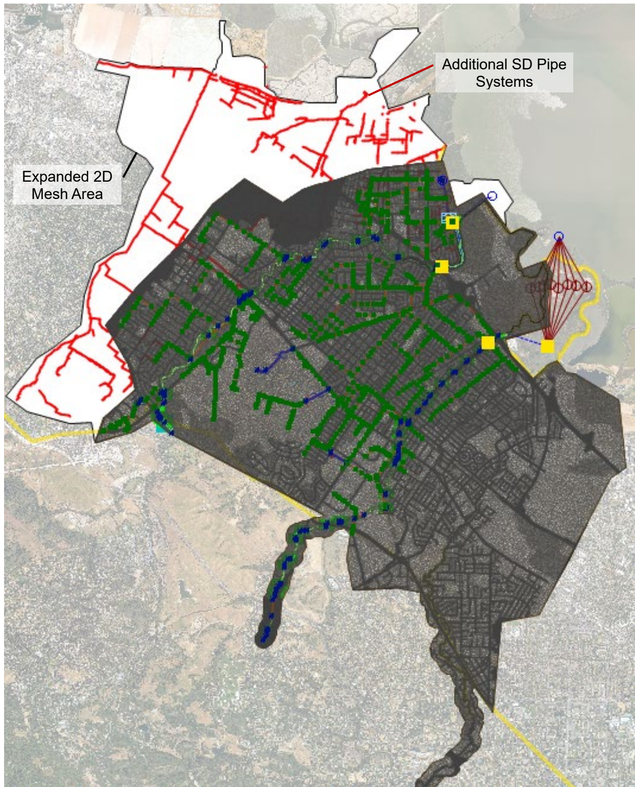
Figure 4-1: Evolution of ICM Geometry
