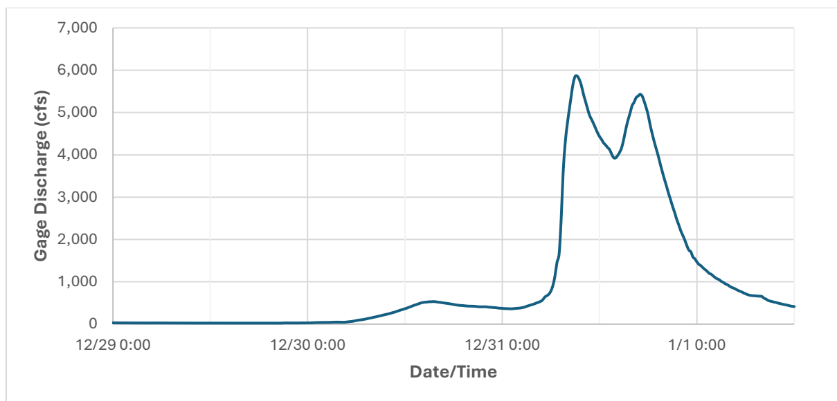
Figure 3-5: Stanford Gage Hydrograph for NYE22
