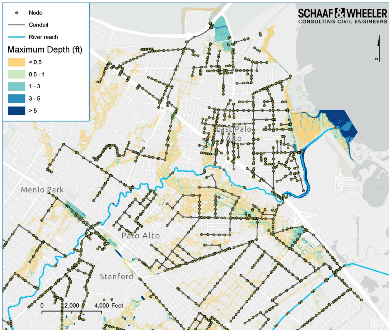
Figure 5-2: NYE22 Flood Depth Result
