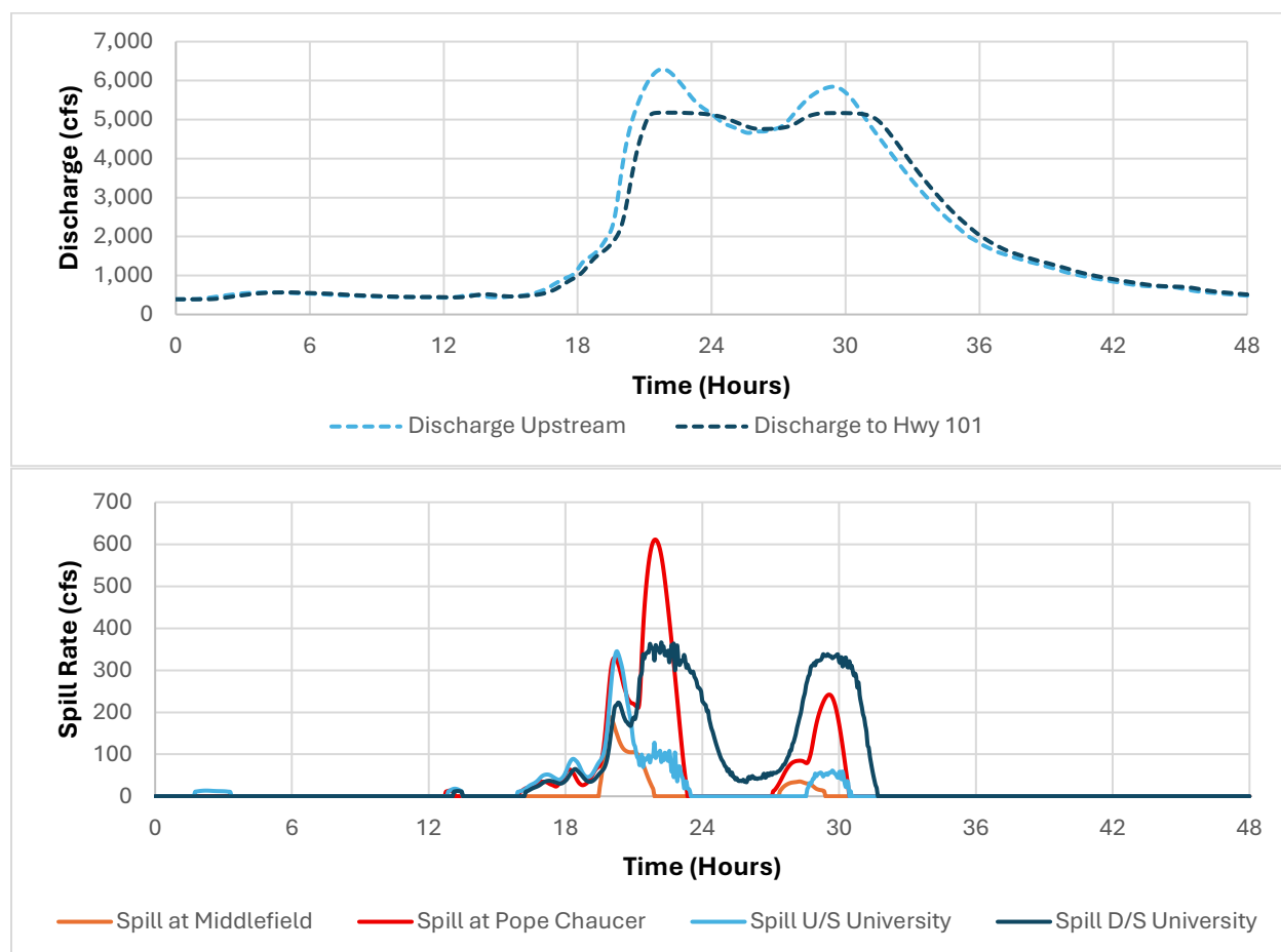
Figure 5-11: NYE22 Spill Hydrographs
