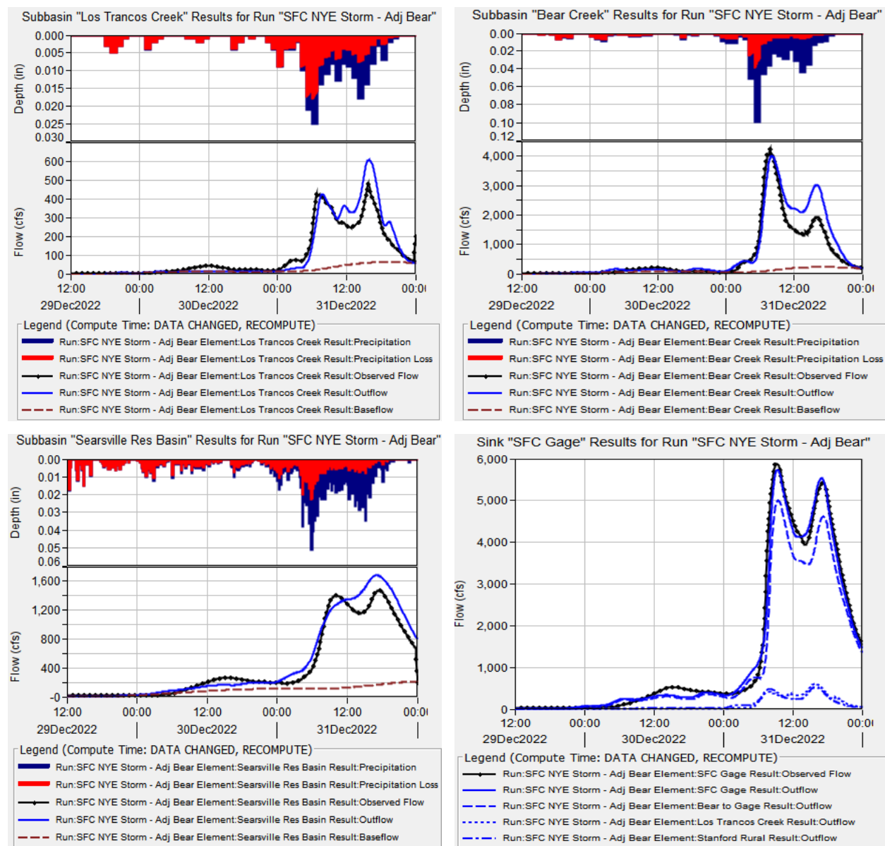
Figure 3-7: Baseflow Calibration Results
