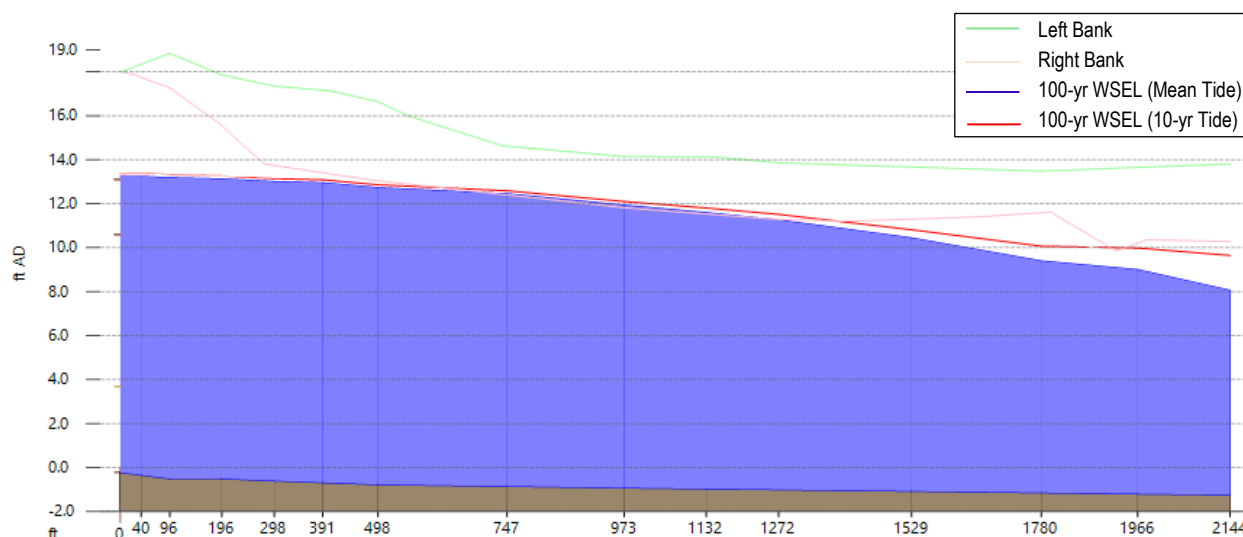
Figure 5-16: Tidal Boundary Sensitivity with 100-year Fluvial Runoff
