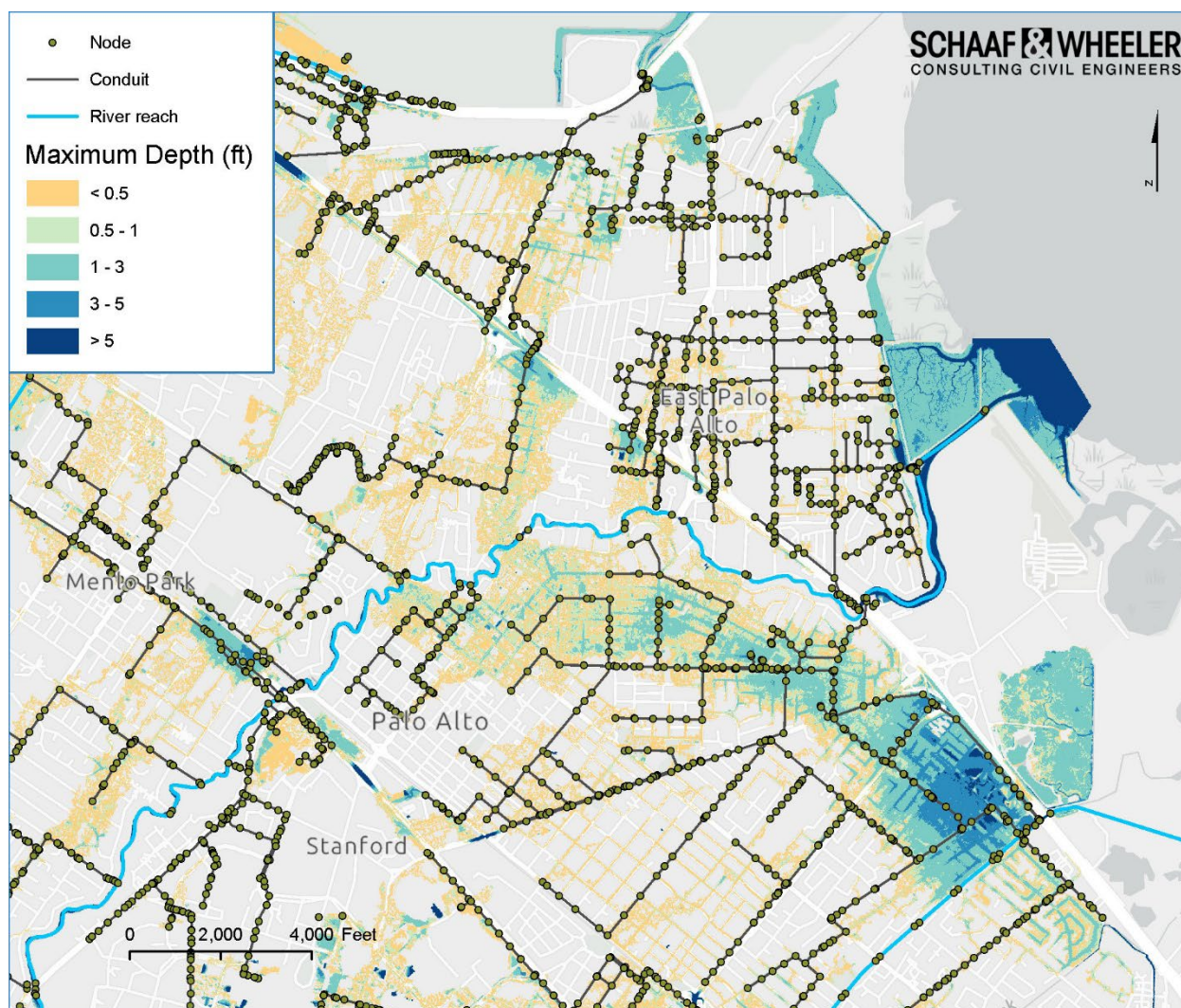
Figure 5-14: 100-year Design Event Flood Depths
