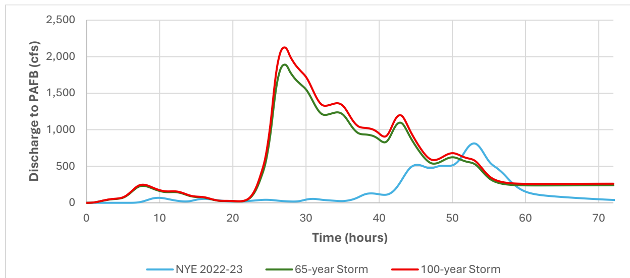
Figure 3-11: Adobe-Barron Design Hydrographs
