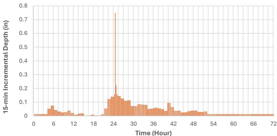
Figure 3-3: 100-year Design Storm Hyetograph for Bear Creek
