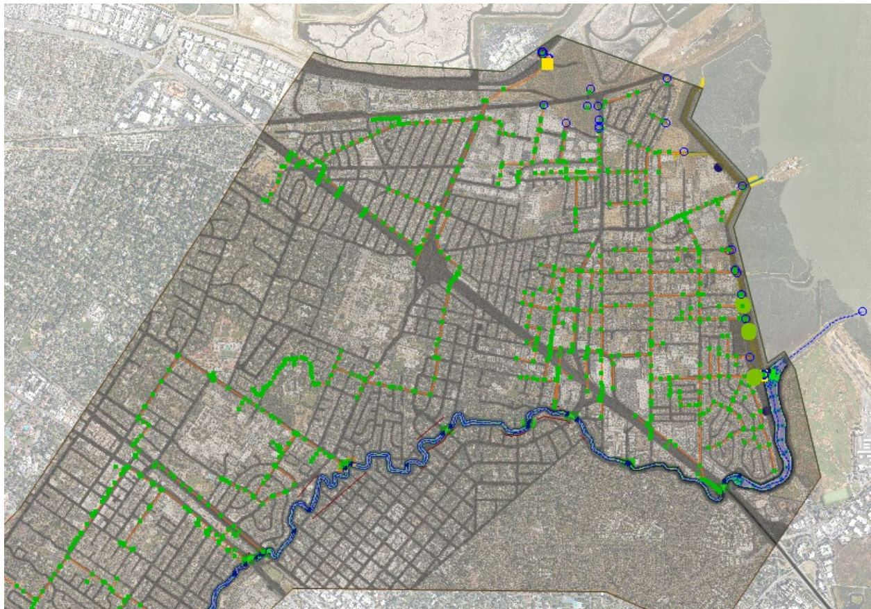
Figure 4-2: SAFER Bay ICM Geometry
