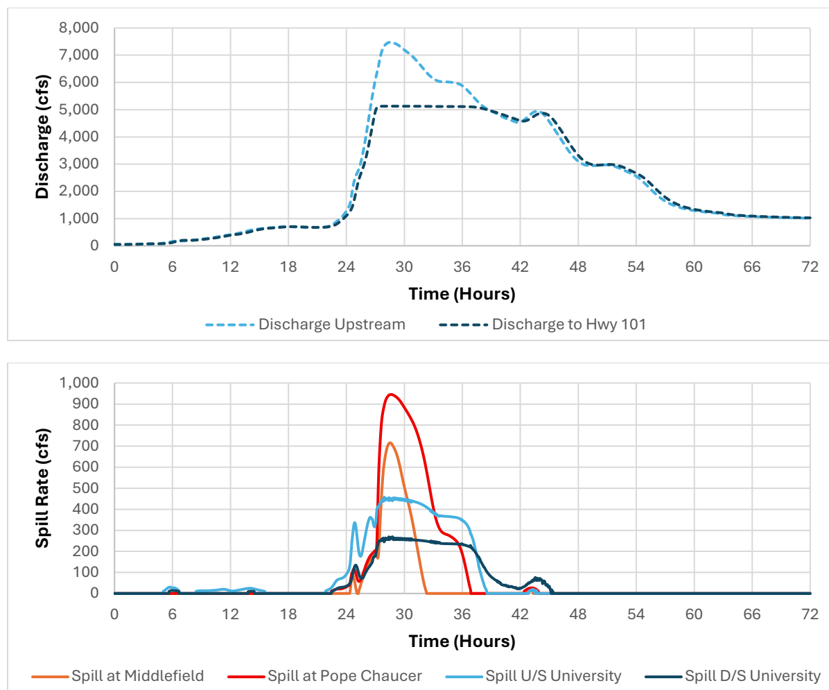
Figure 5-13: 70-year Design Storm (7,200 cfs) Hydrographs
