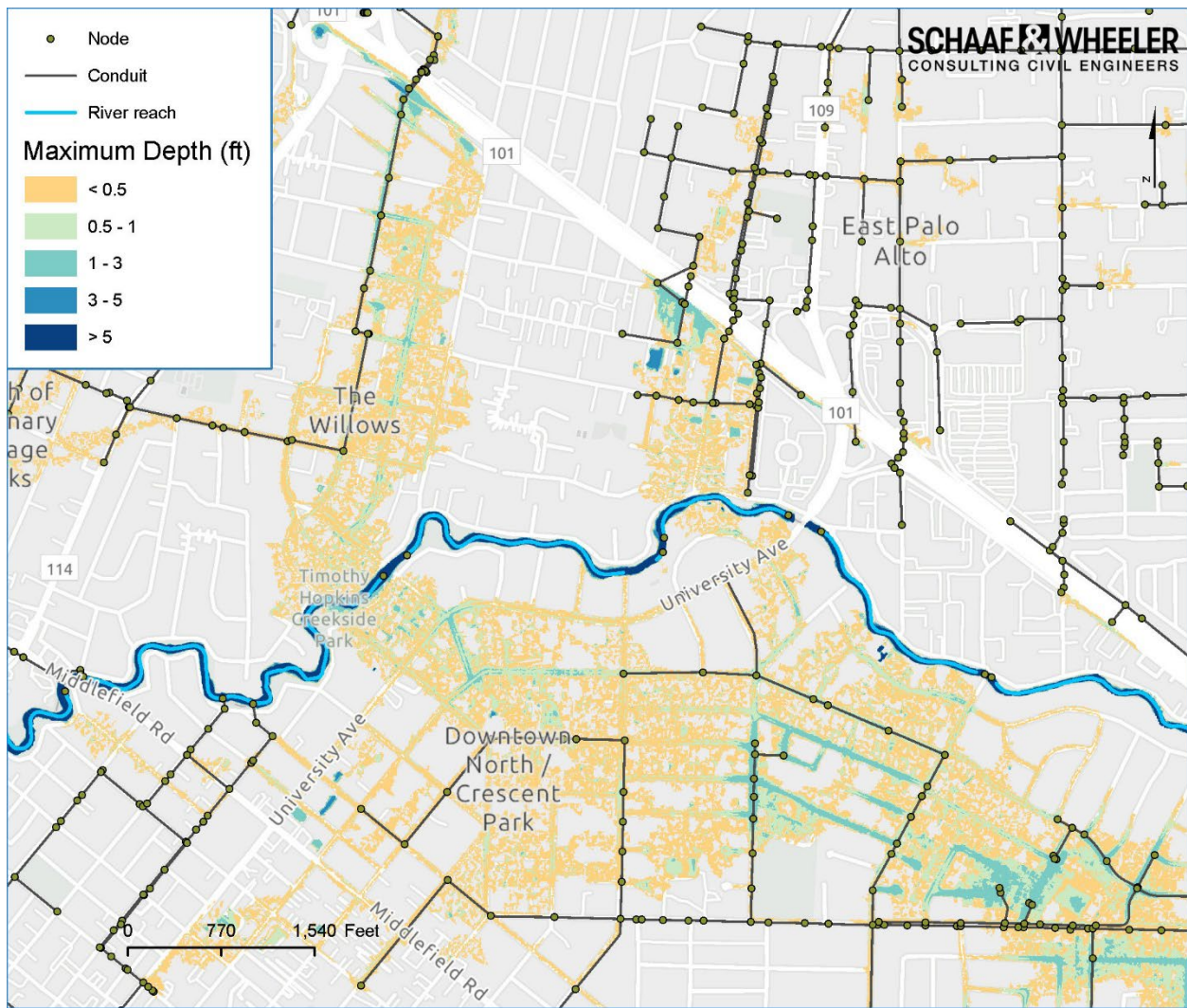
Figure 5-3: NYE22 Flood Depths – Middlefield Road to Highway 101
