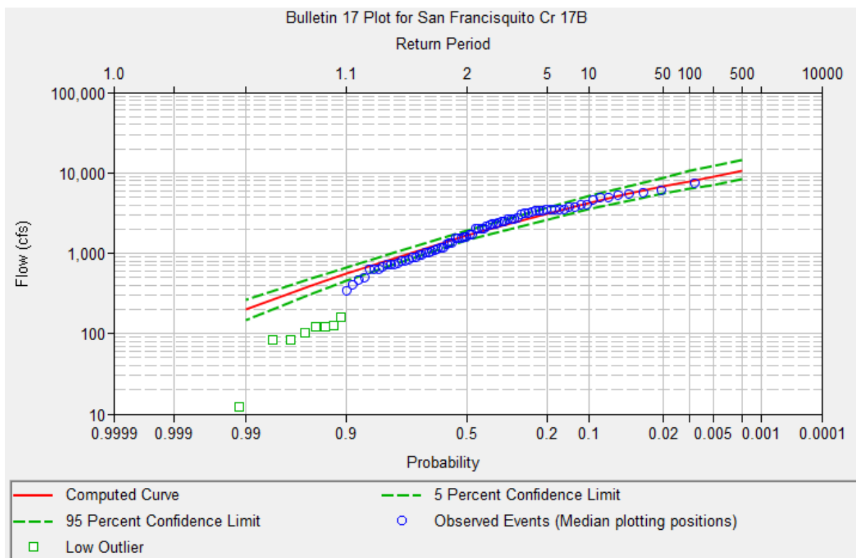
Figure 3-4: San Francisquito Creek Flood-Frequency Analysis
