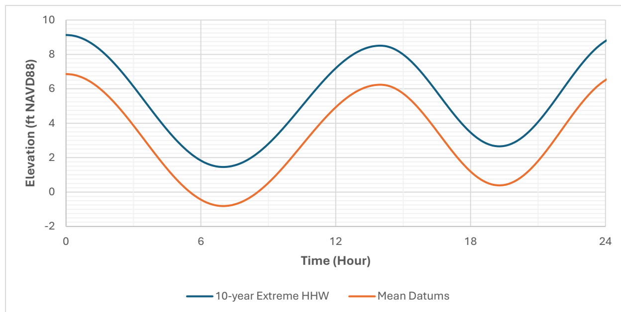
Figure 3-15: Synthetic Mean and 10-year Tide Cycles
