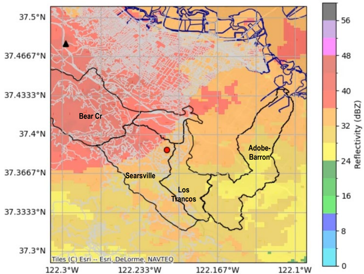
Figure 3-12: NEXRAD Reflectivity During NYE22
