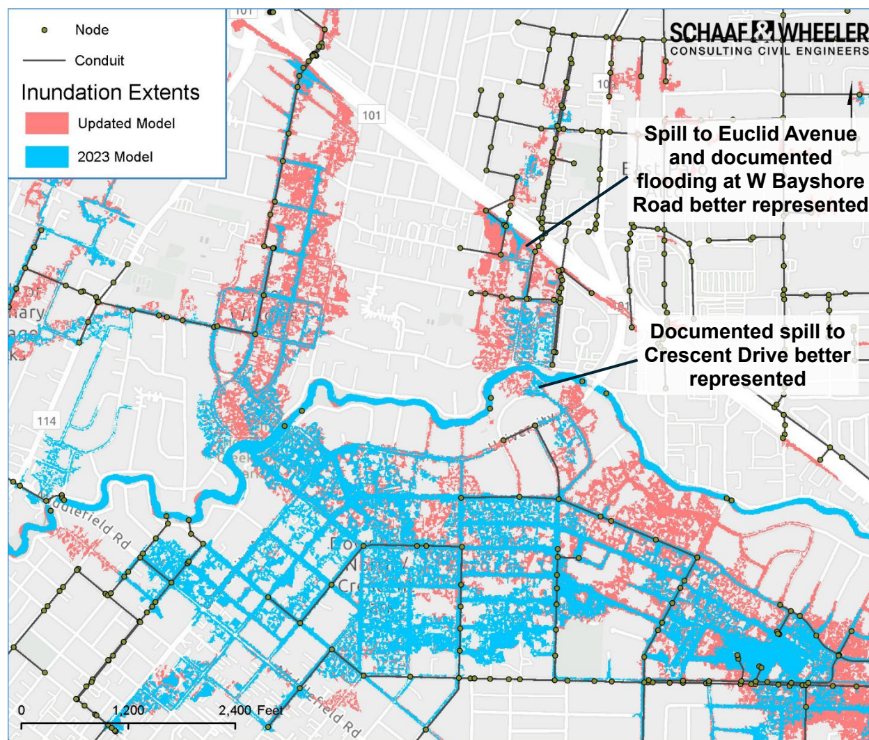
Figure 5-5: Direct Comparison of Modeled Inundation Extents for NYE22 Event
