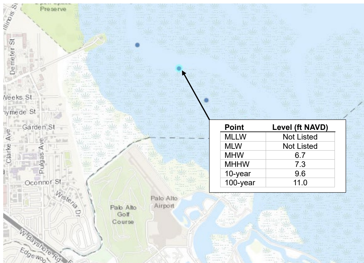
Figure 3-13: Tidal Datums Near San Francisquito Creek Mouth
