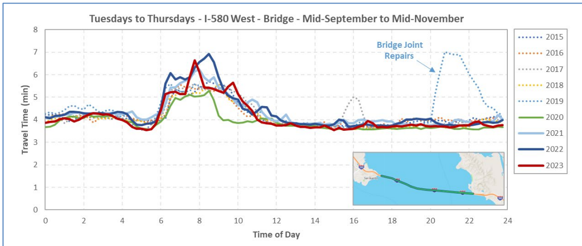
Figure 8-73: Travel Times –Bridge WB – Midweek, Fall 2015-2023
