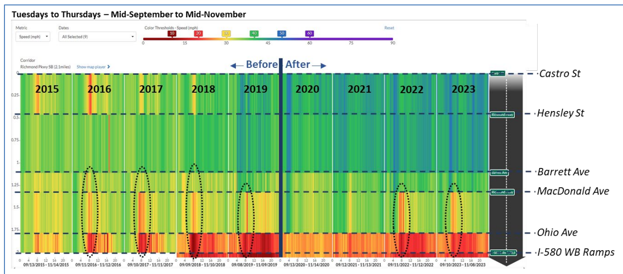
Figure 8-82: Speed Maps – Richmond Parkway SB – Midweek, Fall 2015-2023
