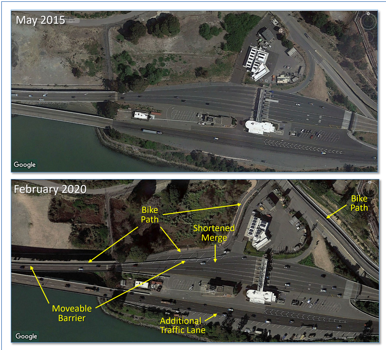
Figure 2-20: Modification of Richmond Approach
